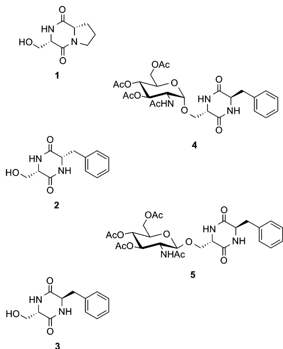
Figure 1. Diketopiperazines and O -glycosylated analogs prepared by solution-phase synthesis.
