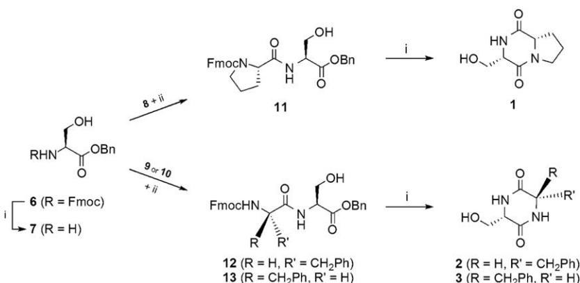
Scheme 1. Synthesis of diketopiperazines 1 , 2 , and 3 . Reagents and conditions: (i) 20% piperidine/DMF, rt; (ii) PyBOP, HOBT, DIEA/MeCN, rt.
