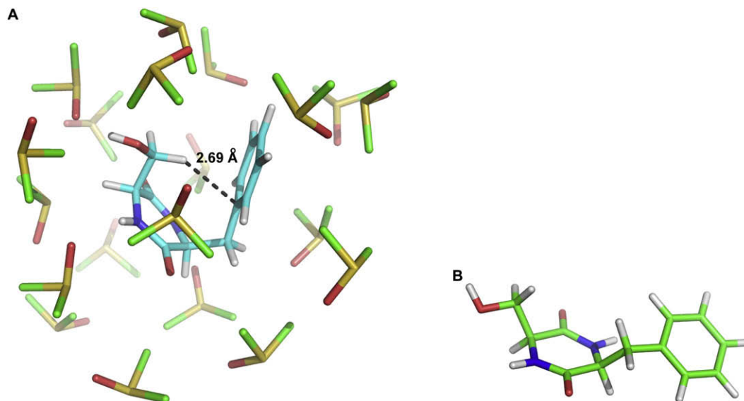
Figure 2. Structures of diketopiperazine 2 in the two main low-energy conformations. In (A), the folded conformer solvated (one layer) with DMSO, and the overall system geometry-optimized at AM1 level of calculation. After the simulation, short distance of 2.69 Å was obtained for the CH/π contact, here represented by a dashed line. Hydrogen atoms of the DMSO molecules were omitted for the sake of the clarity. In (B), the extended conformer geometry-optimized in gas phase at B3LYP/6-31G* level of calculation is shown.
