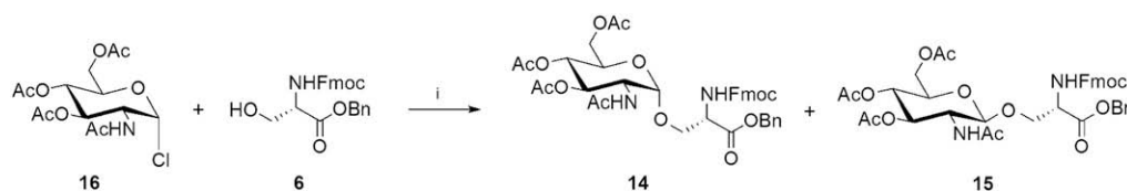
Scheme 2. Synthesis of the building blocks 14 and 15 by glycosylation reaction. Reagents and conditions: (i) \text{HgBr}_2 , DCE, reflux 9 h.
