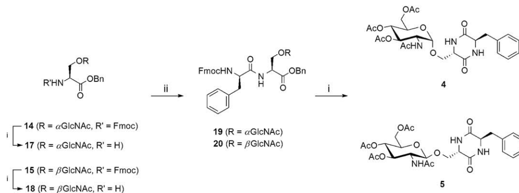
Scheme 3. Synthesis of diketopiperazines 4 and 5 . Reagents and conditions: (i) 20% piperidine/DMF, rt; (ii) Fmoc-D-Phe-OH ( 10 ), PyBOP, HOBt, DIEA/MeCN, rt.
